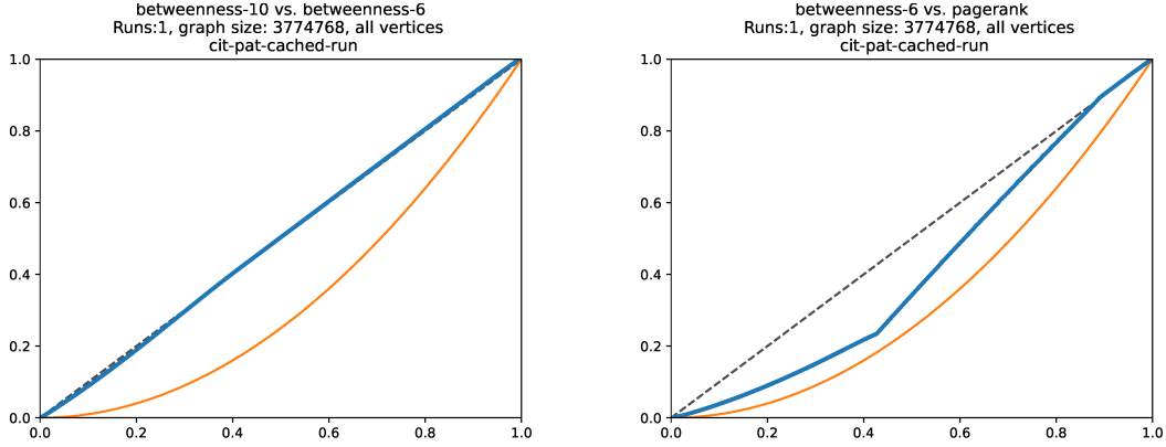
FIGURE 10. CCC for betweenness6 versus betweenness10 , and betweenness6 versus PageRank, respectively, for the “Patent” network [51].
