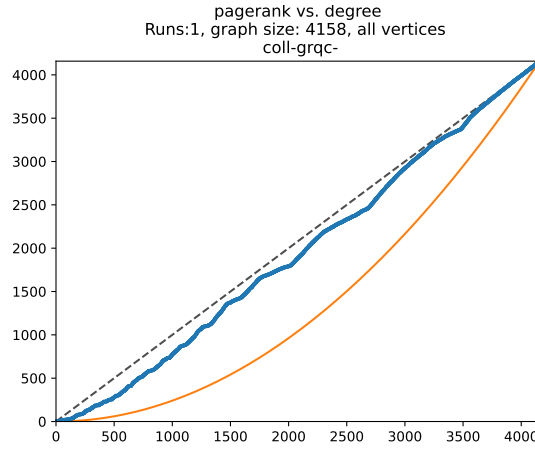
FIGURE 15. CCC for PageRank versus degree for the collaboration network [51].
