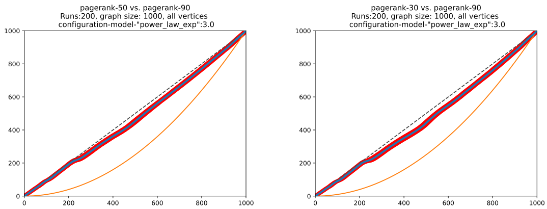
FIGURE 20. CCC for PageRank with damping factors 0.5 versus 0.9, and 0.3 versus 0.9, respectively, for the artificial network.
