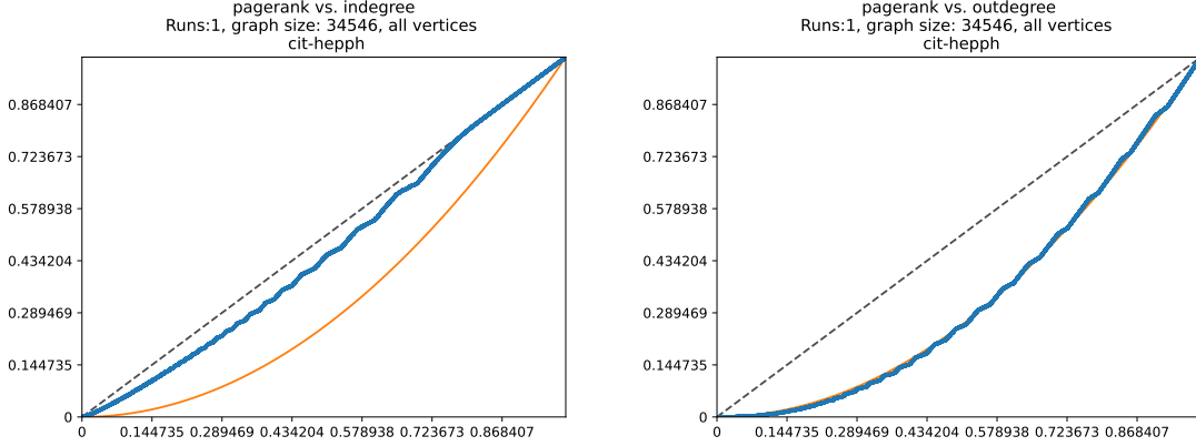
FIGURE 1. CCC for PageRank versus in-degree, and PageRank versus out-degree, for the “hep-ph” citation network [37].
