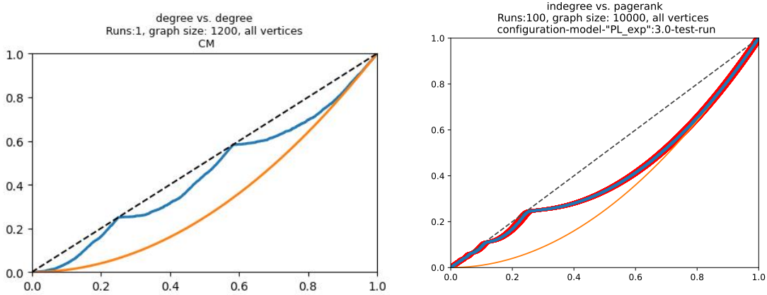
FIGURE 11. Effect of alternative tie-breaking rules on the CCC: CCC of degree versus degree for an undirected configuration model with 500 vertices of degree 3, 400 of degree 4, and 300 of degree 5, with the random tie-breaking rule, and PageRank versus indegree for a directed configuration model with an alternative tie-breaking rule. Compare with Figure 4.
