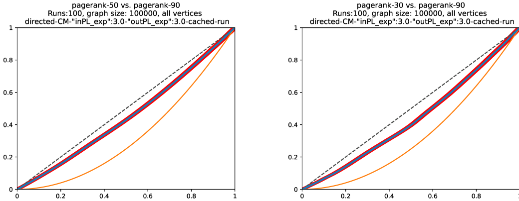
FIGURE 5. CCC for PageRank with damping factors 0.5 versus 0.9, and 0.3 versus 0.9, respectively, for the artificial network.
