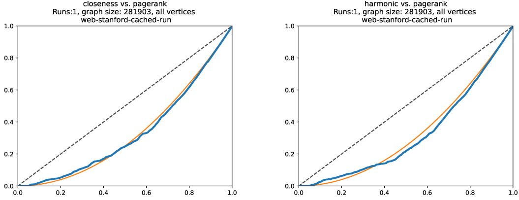
FIGURE 23. Stanford web graph: CCC for closeness versus PageRank (left) and harmonic versus PageRank (right). Both curves are close to x^2 , indicating near-independence.
