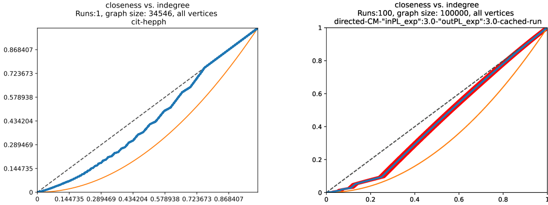
FIGURE 8. CCC for closeness versus in-degree, for the “hep-ph” citation network [37] and the artificial network.
