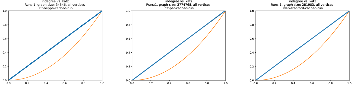
FIGURE 6. CCC for in-degree versus Katz centrality for the “hep-ph” citation network [37], the “Patent” network [51], and Stanford web graph dataset [53].
