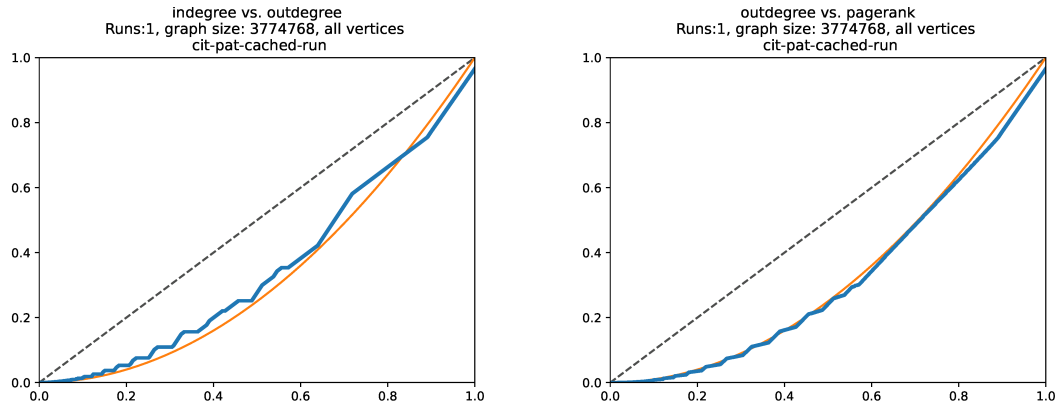
FIGURE 25. Patent network: CCC for in-degree versus out-degree (left) and out-degree versus PageRank (right). Both curves are close to x^2 , indicating near-independence.
