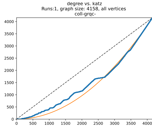
FIGURE 16. CCC for eigenvector versus PageRank, and degree versus Katz centrality, respectively, for the collaboration network [51].
