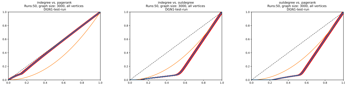
FIGURE 14. CCC for in-degree versus PageRank, in-degree versus out-degree, and out-degree versus PageRank for the [19].
