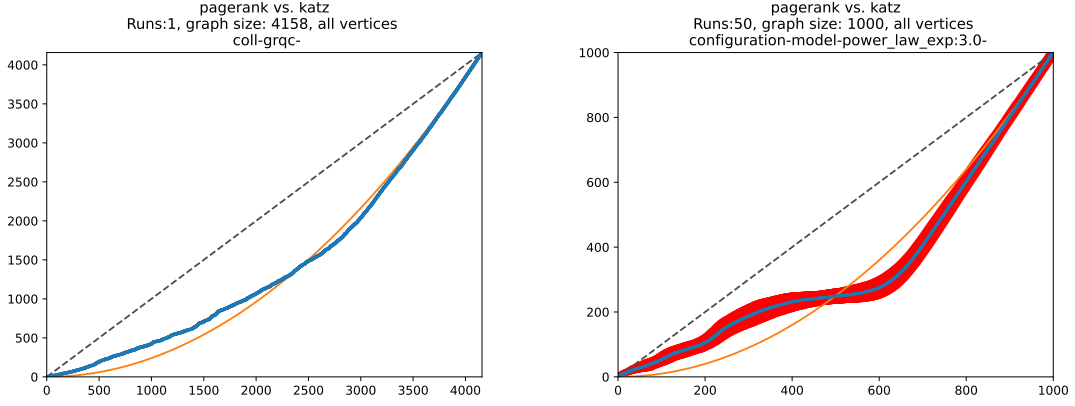
FIGURE 21. CCC for PageRank versus Katz, for the collaboration network [51] and the artificial network.
