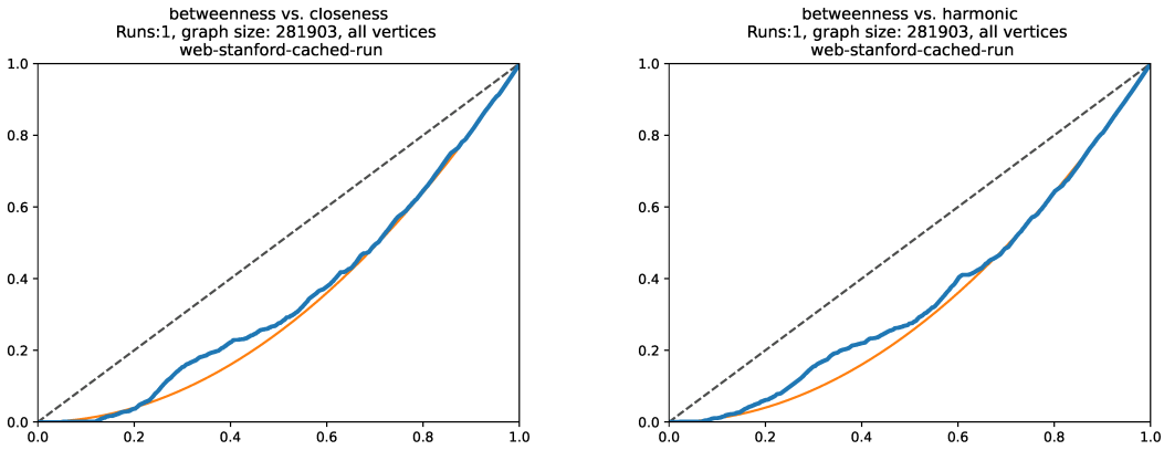
FIGURE 22. Stanford web graph: CCC for betweenness versus closeness (left) and betweenness versus harmonic (right). Both curves are close to x^2 , indicating near-independence.
