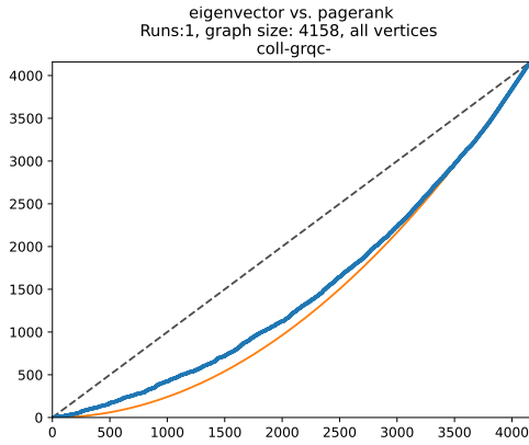
FIGURE 16. CCC for eigenvector versus PageRank, and degree versus Katz centrality, respectively, for the collaboration network [51].
