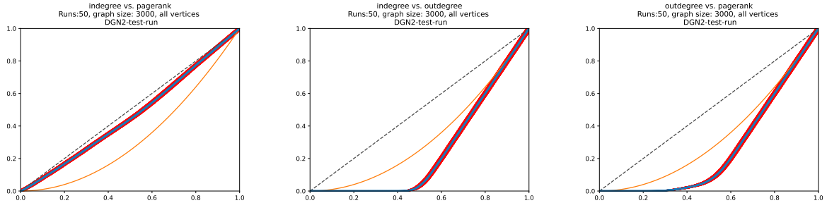
FIGURE 13. CCC for in-degree versus out-degree, in-degree versus PageRank, and out-degree versus PageRank for the directed product graphon where in-degrees and out-degrees are maximally different. In-degree and PageRank are almost identical, out-degree is close to maximally different from in-degree and PageRank.
