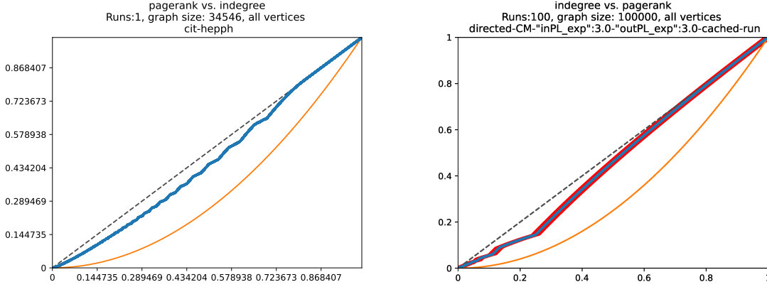
FIGURE 4. CCC for PageRank versus in-degree, for the “hep-ph” citation network [37] and the artificial network.
