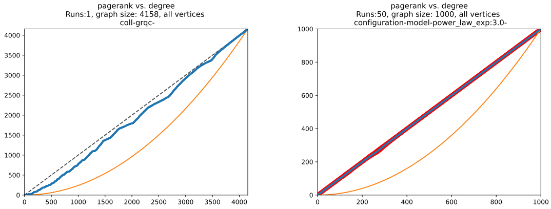
FIGURE 19. CCC for PageRank versus degree for the collaboration network [51] and the artificial network.
