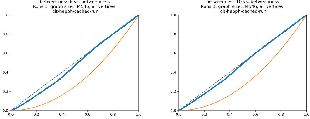
FIGURE 9. CCC for betweenness versus betweenness6 and betweenness10 , respectively, for the “hep-ph” citation network [37].
