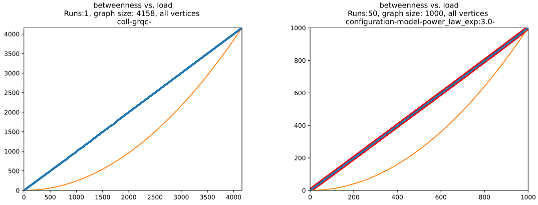
FIGURE 18. CCC for betweenness versus load centrality for the collaboration network [51] and the artificial network.
