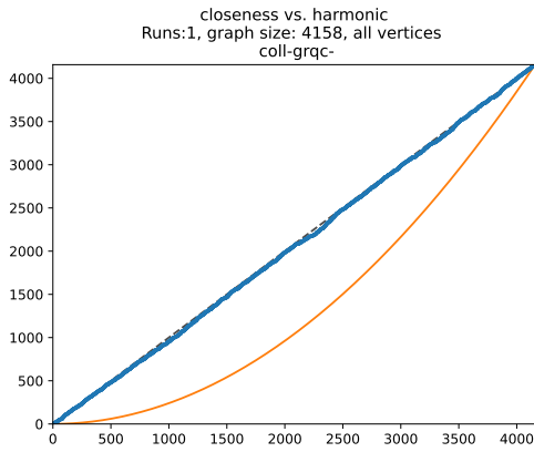
FIGURE 17. CCC for closeness versus harmonic centrality for the collaboration network [51] and the artificial network.
